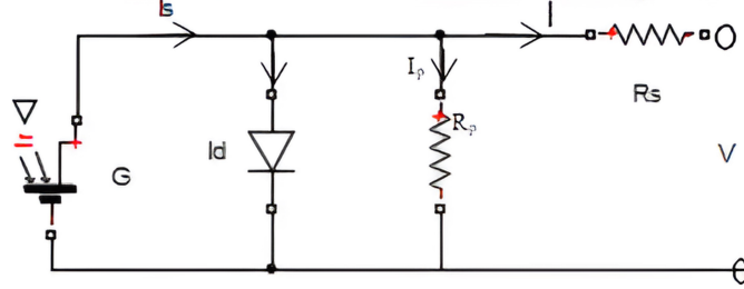
Figure 1: Single diode model with R_s and R_p .
