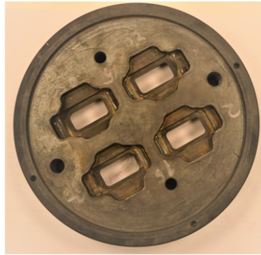
Figure 1: Extrusion die for aluminium alloy profiles [34].
