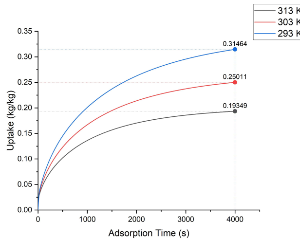
Figure 7: Comparison of the amount of vapor adsorbed by the bed at different cooling water temperatures.
