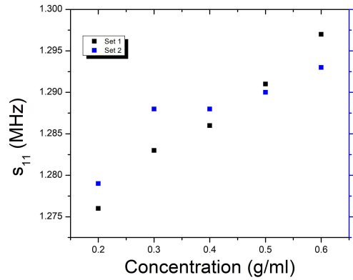
Fig. 12. Stability graph of frequency for the repeated experiment.
