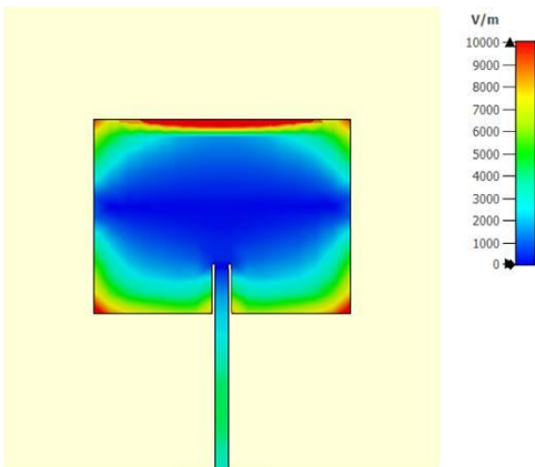
Fig. 3. Electric field distribution on the patch.
