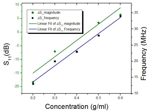
Fig. 9. Regression analysis of S_{11} frequency and magnitude with respect to glucose concentrations.
