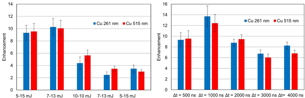
Fig. 9. Maximum enhancement of the LIBS signal for different energies of DP pulses (left) and for different gate delays (right).
