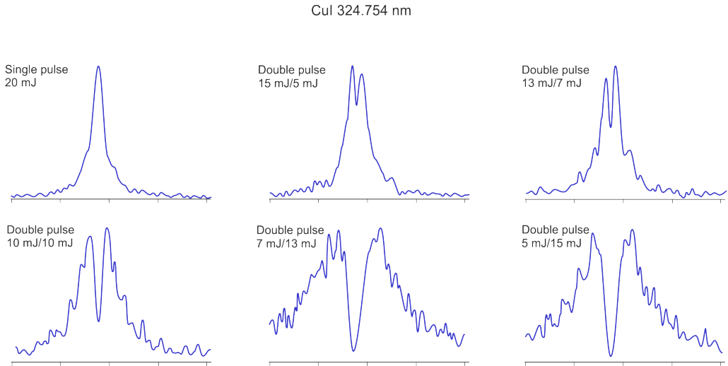
Fig. 5. Cu I 324.754 nm line profile. All spectra were taken for 500 ns gate widths and 500 ns gate delays after the laser pulse (the second one in the DP-LIBS mode). The wavelength scale starts at 324.4 nm and ends at 325.2 nm.
