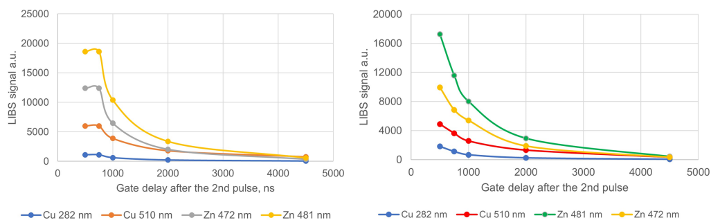
Fig. 4. 500 ns LIBS signals for various gate delays and 250 ns (left) and 500 ns (right) inter-pulse delays.
