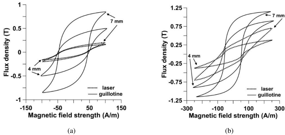
Fig. 4. Measured hysteresis loops for for strips of two widths (M300-35):
