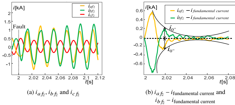
Fig. 18. The simulation result of two-phase short-circuit of converter transformer valve-side bushing
