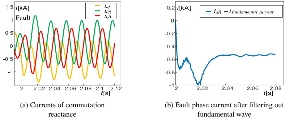
Fig. 17. A-phase grounding with fault resistance R_f = 100 \Omega on the valve side bushing
