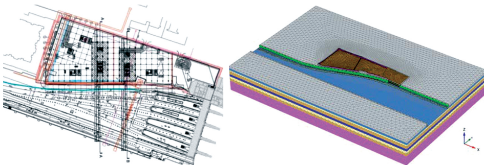
Fig. 5. Deep excavation in the vicinity of active railway tracks: situational plan (left) and spatial model of the subsoil and objects (right)
