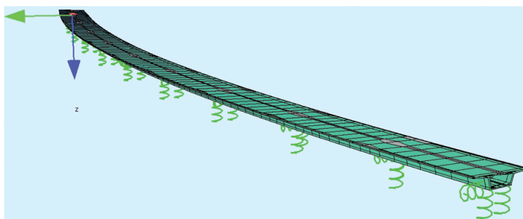
Fig. 16. Visualization of the model of the superstructure of the left roadway
