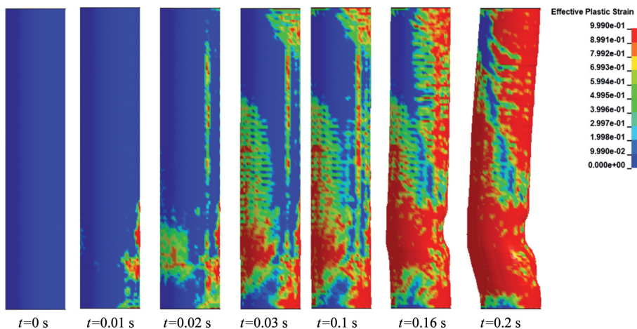
Fig. 8. Damage process of the bridge pier
