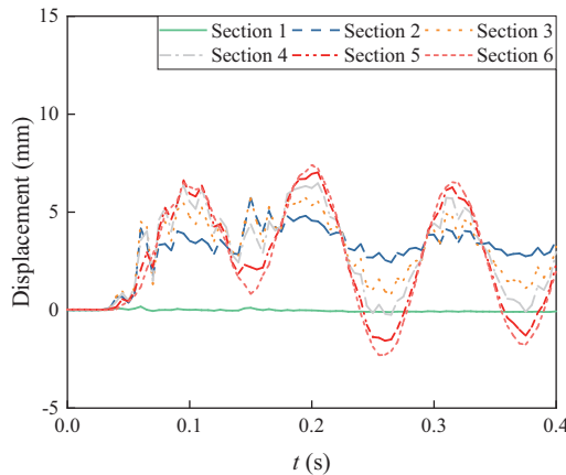
Fig. 9. Time history of displacement
