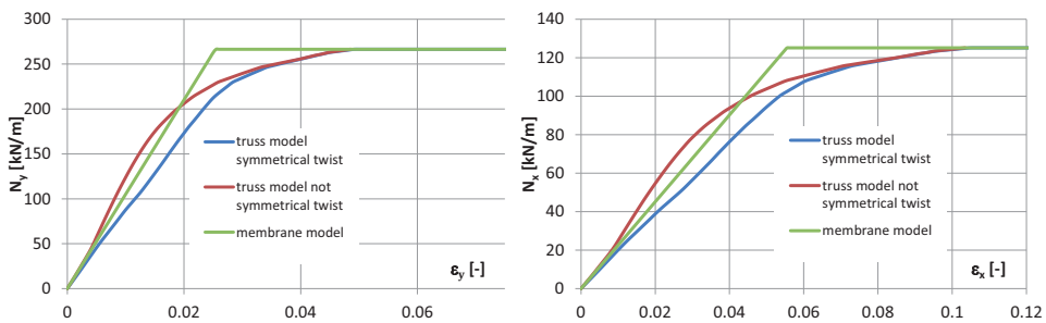
Fig. 16. Comparison of load-strain curves obtained from the truss model of the repeatable cell of the mesh and the membrane model
