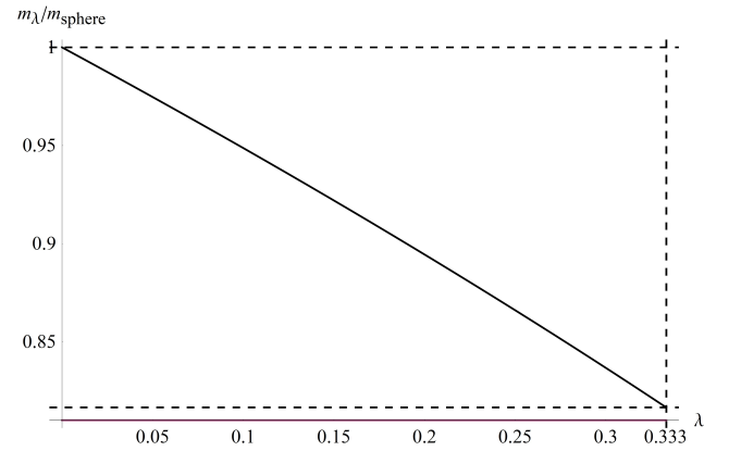
Fig. 3. Dependence of quarter-meridian length m_\lambda of deformed sphere scaled by quarter-meridian length m_{\text{sphere}} = \pi R/2 of equivalent sphere with radius R on deformation parameter \lambda \in [0, 1/3] . Gridlines (dashed) are \lambda = 1/3 , m_\lambda/m_{\text{sphere}} = 0.816\,496\,581\dots , and m_\lambda/m_{\text{sphere}} = 1
