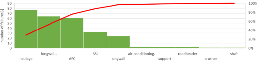
Fig. 7. Pareto chart for the number of electrical failures in shearer longwalls
