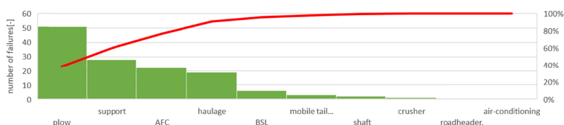
Fig. 19. Pareto chart for the number of mechanical failures in plow longwalls
