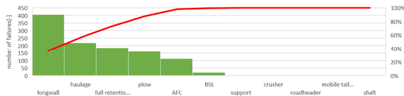
Fig. 13. Pareto chart for the number of mining failures in plow longwalls
