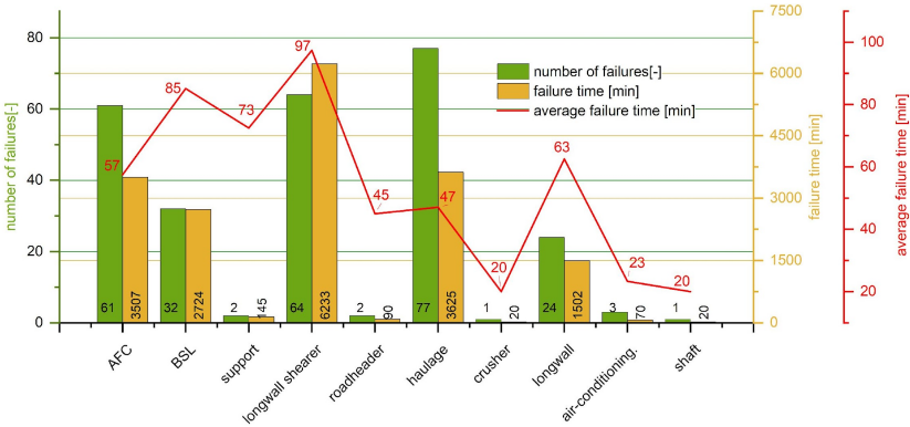
Fig. 6. Number, duration and average duration of electrical failures in shearer longwalls
