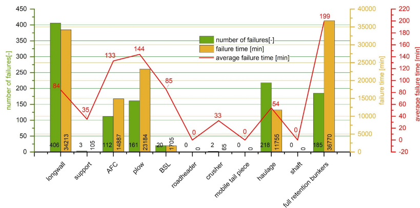
Fig. 12. Number, duration and average duration of mining failures in plow longwalls
