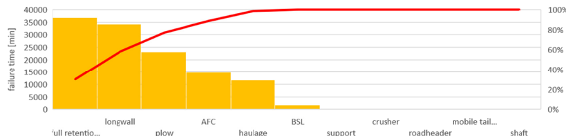
Fig. 14. Pareto chart for the duration of mining failures in plow longwalls
