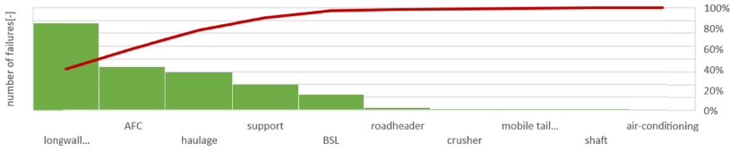
Fig. 10. Pareto chart for the number of mechanical failures in shearer longwalls
