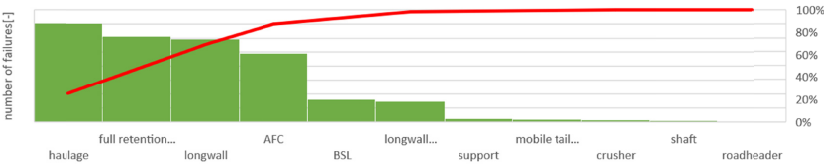
Fig. 4. Pareto chart for the total number of mining failures in shearer longwalls
