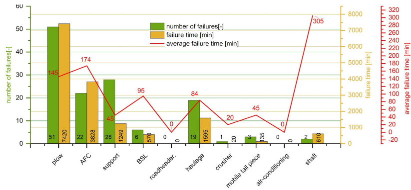
Fig. 18. Number and average duration of mechanical failures in plow longwalls
