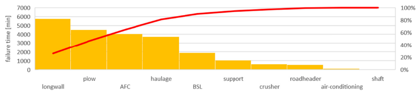
Fig. 17. Pareto chart for the duration of electrical failures in plow longwalls
