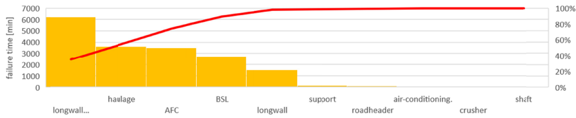
Fig. 8. Pareto chart for the duration of electrical failures in shearer longwalls
