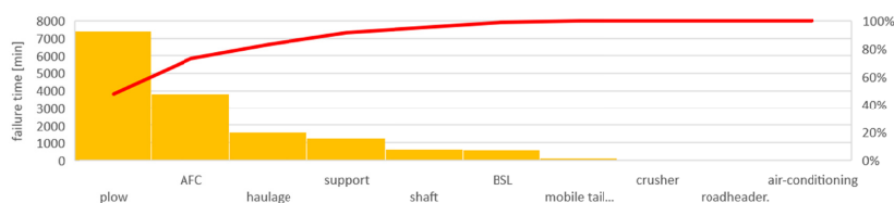
Fig. 20. Pareto chart for the duration of mechanical failures in plow longwalls
