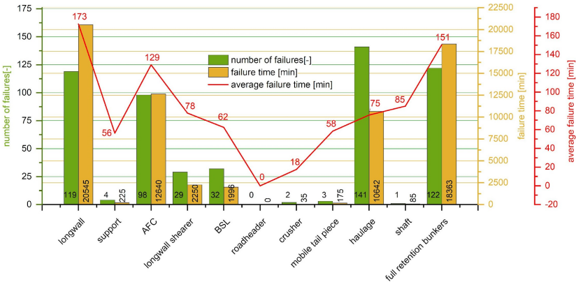
Fig. 3. Number, duration and average duration of mining failures in shearer longwalls
