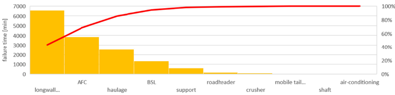
Fig. 11. Pareto chart for the duration of mechanical failures in shearer longwalls
