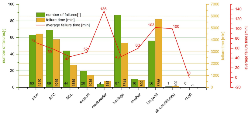
Fig. 15. Number and average duration of electrical failures in plow longwalls
