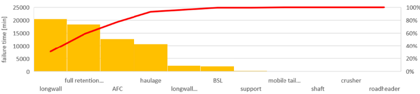
Fig. 5. Pareto chart for the total duration of mining failures in shearer longwalls
