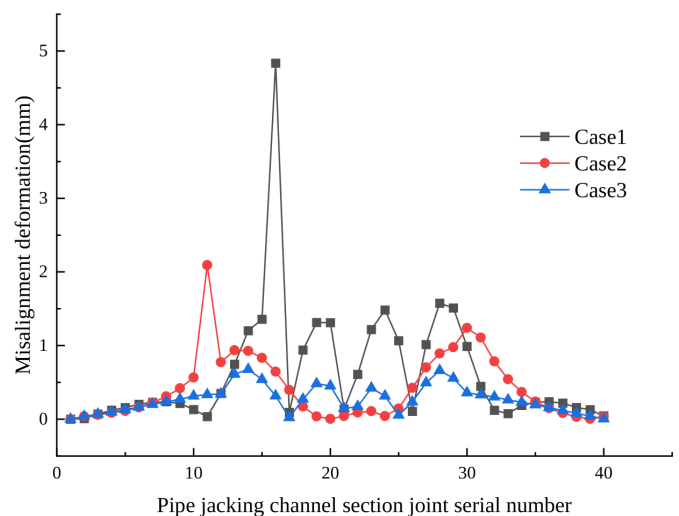
Fig. 13. Misalignment deformation of pipe jacking channel section joints
