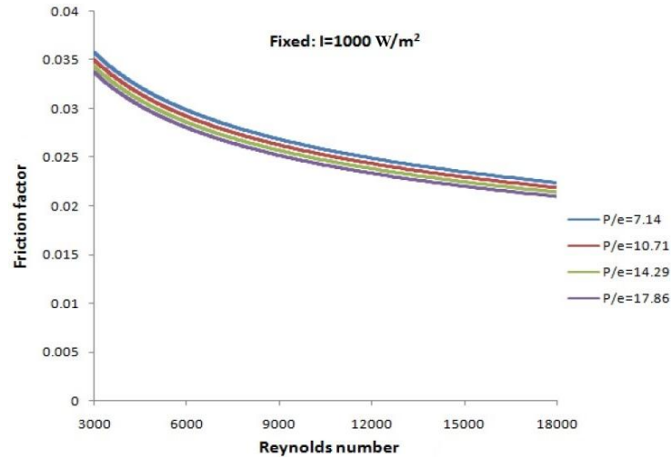
Figure 15: Variation of friction factor ( f ) with Reynolds number ( Re ).
