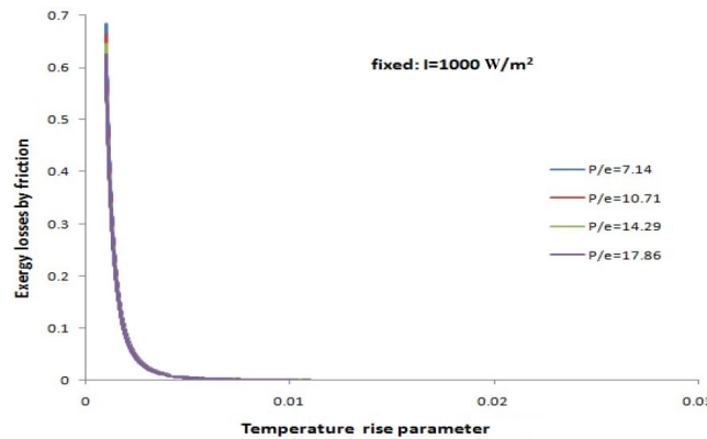
Figure 5: Variation of exergy losses by friction ( El_{\Delta p} ) with temperature rise parameter ( \Delta T/I ).
