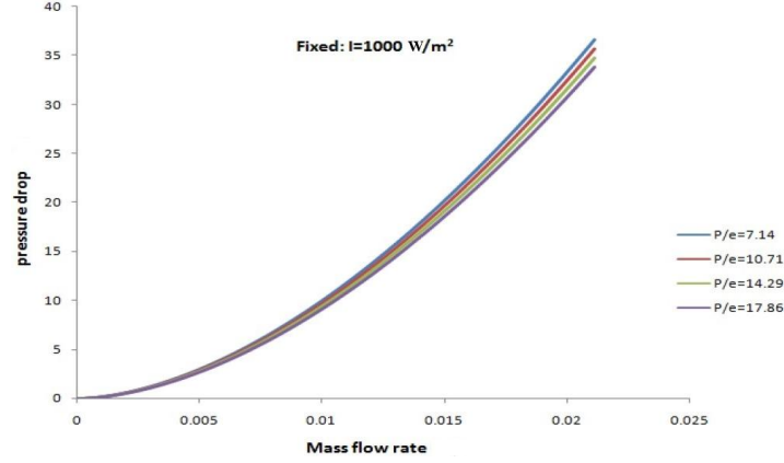
Figure 12: Variation of pressure drop ( \Delta p ) with mass flow rate ( \dot{m} ).
