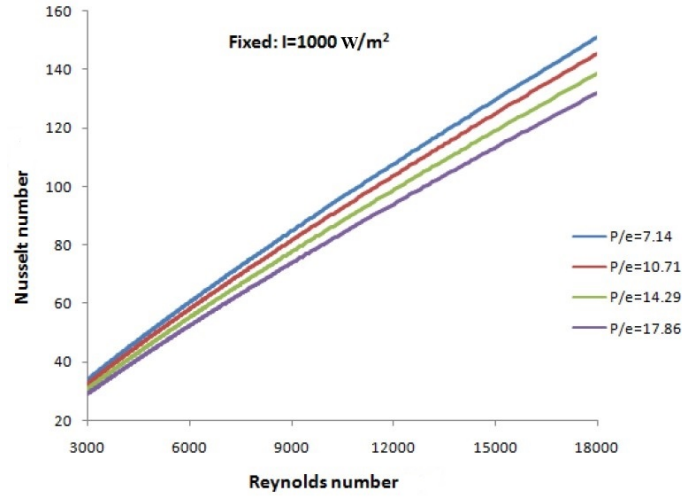
Figure 14: Variation of Nusselt number with Reynolds number.
