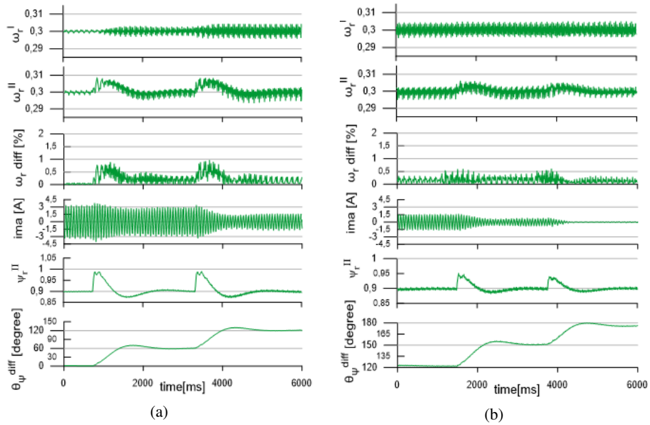
Fig. 11. Rotor speeds, the rotors' speed difference, inverter common phase current, the estimated flux component and the mutual flux angle values under a step change in the mutual flux angle: from 0 to 60 and then to 120 degrees (a); from 120 to 150 and then to 175 degrees (b)
