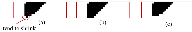
Fig. 12. Optimized topology from deterministic optimization (a); optimized topology from robust optimization (b); distorted topology from (a) (c)
