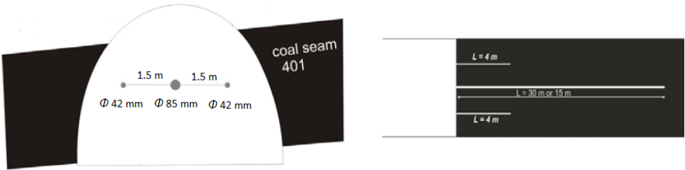
Fig. 6. Drilling layout for water injection tests in the roadway coal face in the 401 coal seam
