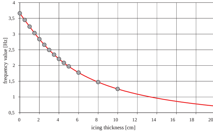
Fig. 13. The fundamental natural frequency of the model and its hyperbolic dependence on the thickness of the ice layer (also marked with a red line in Fig. 12)
