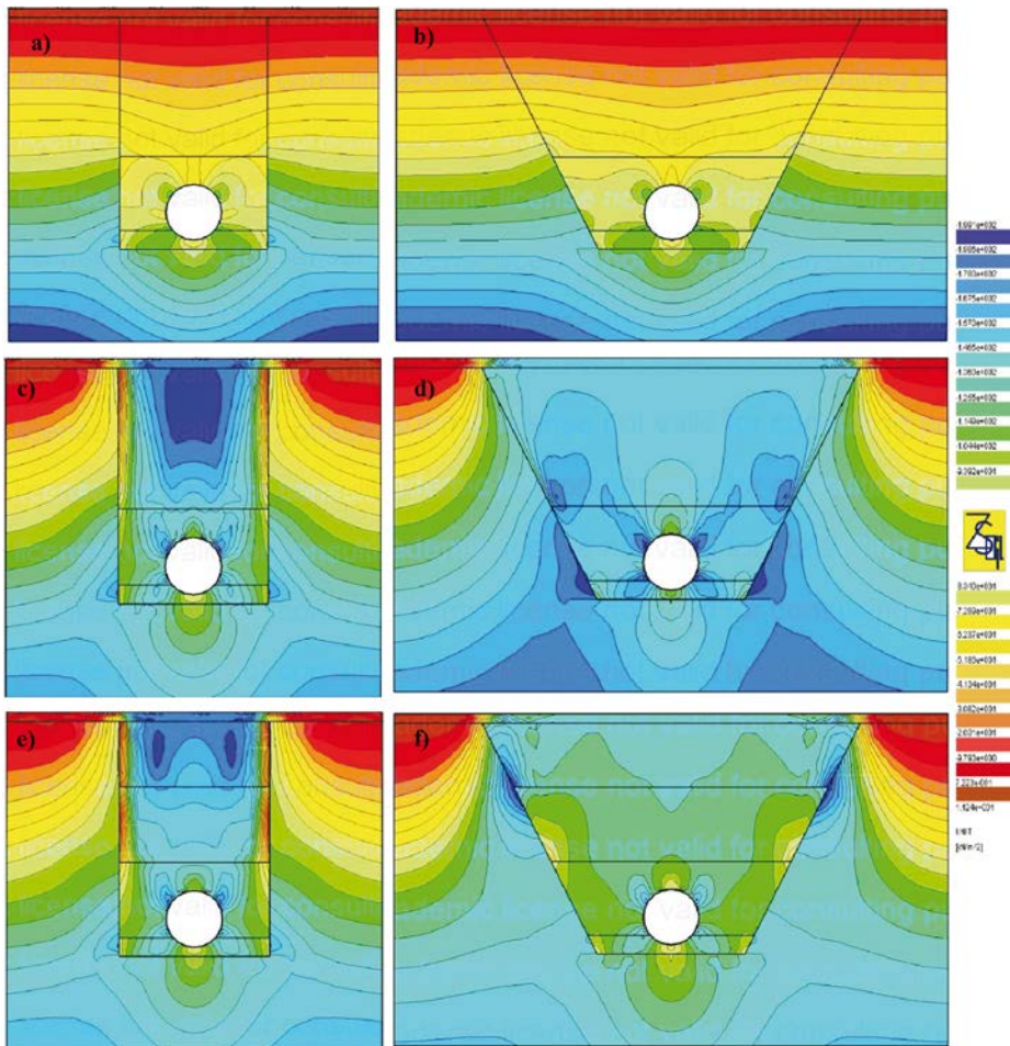
Fig. 7. Maps of vertical stress: a) 600_SDR41_N_SOIL ( t = 0 ), b) 600_SDR41_W_SOIL ( t = 0 ), c) 600_SDR41_N_SOIL ( t = 5 ), d) 600_SDR41_W_SOIL ( t = 5 ), e) 600_SDR41_N_LECA ( t = 5 ), f) 600_SDR41_W_LECA ( t = 5 )
