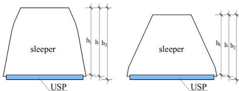
Fig. 4. Positioning of USP at the bottom of the rail support in vertical plane. Symbols: h – nominal height of the rail support; h_1 – net height of the rail support (without taking into account the part of the pad embedded inside); h_2 – total height of the rail support with USP
