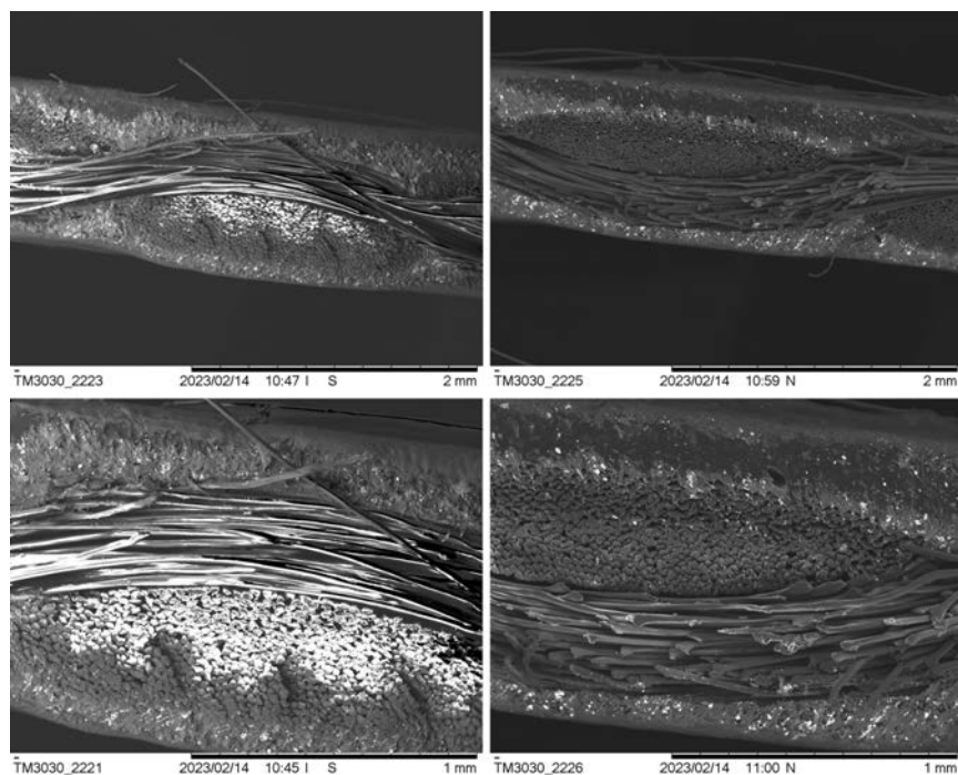
Fig. 5. SEM microscopic images – C-type fabric
