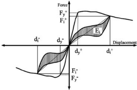
Fig. 15. Cyclic stiffness calculation parameters
