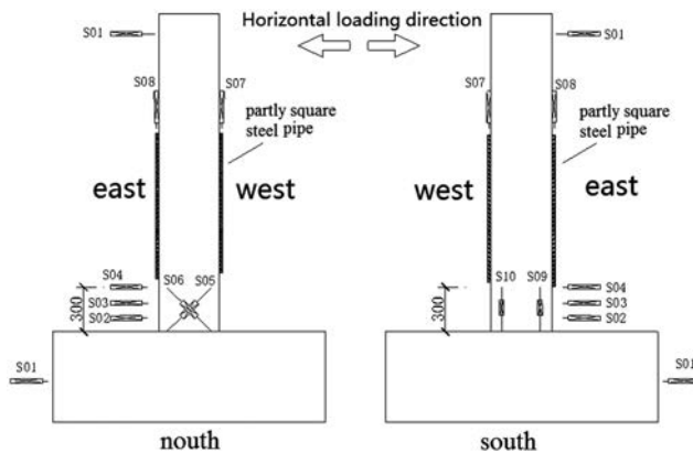
Fig. 6. Typical LVDTs arrangement on specimens
