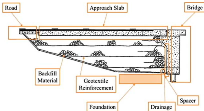
Fig. 2. Approach and Departure Slabs Endanger Drivers [12]
