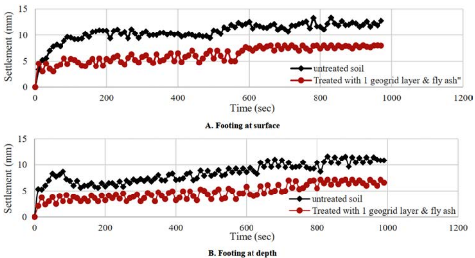
Fig. 8. Settlement against time for treated and untreated with fly ash and one geogrid layer models with velocity = 6 mm/sec and various depth
