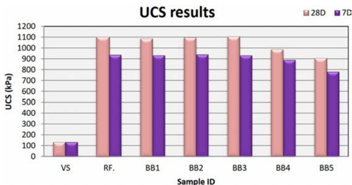
Fig. 5. Un-confined compressive strength test finding for both treated and untreated soft soil
