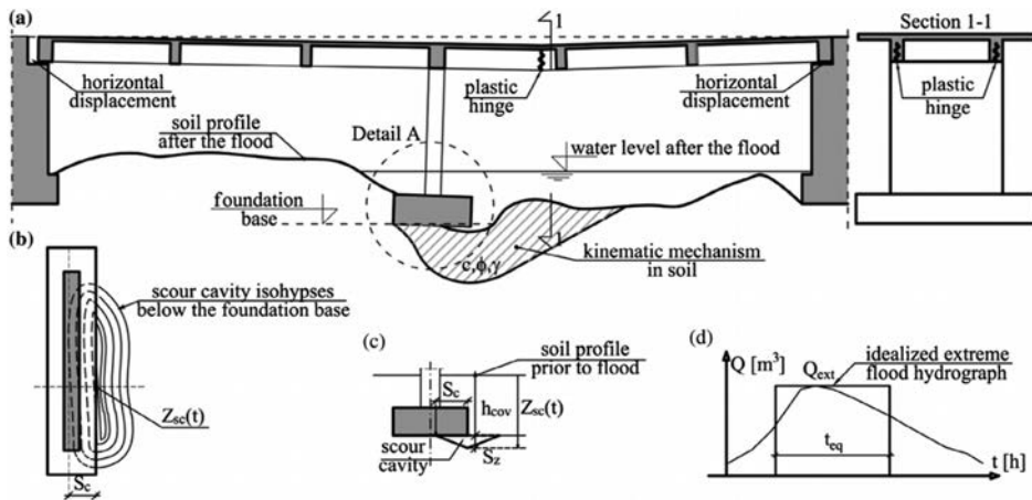
Fig. 1. (a) Bridge failure mode in the longitudinal direction; (b) a local scour cavity at the affected pier foundation; (c) detail a – the cavity approximation; (d) an idealized extreme flood hydrograph [8]
