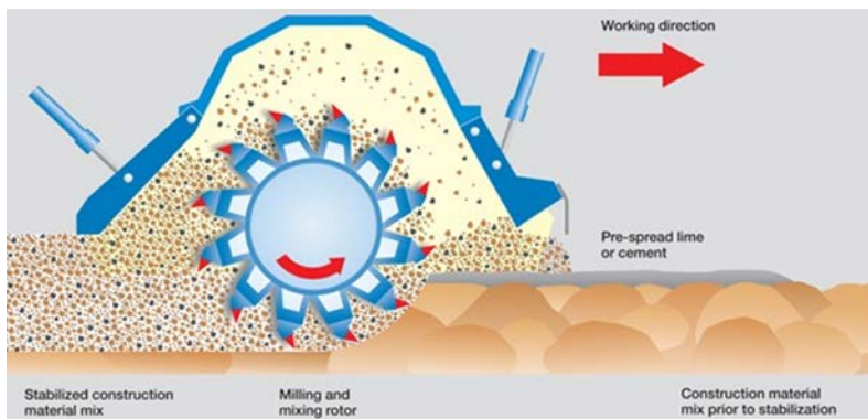
Fig. 3. Soil Stabilization Mechanism [39]
