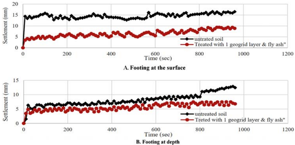
Fig. 7. Settlement against time for treated and untreated with fly ash one and geogrid layer models with velocity
