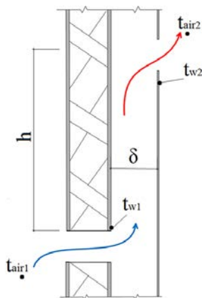
Fig. 1. A simplified model of hot air flows in the Trombe Wall
