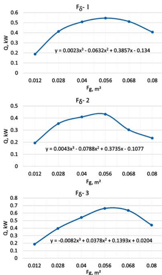
Fig. 6. The amount of heat received with the help of the Trombe Wall
