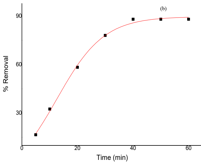
Fig. 3. (a) Effect of time of Fe (III) adsorption by Peganum Harmala., (b) Effect of time for removal Fe (III) by Peganum Harmala.
