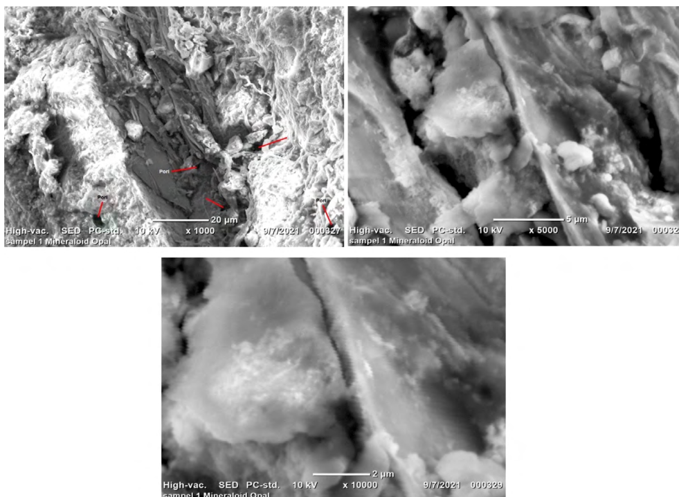
Fig. 4. Image of rock sample 1 with magnification of 1,000×, 5,000×, and 10,000× Source: Indonesian Muslim University Laboratory
