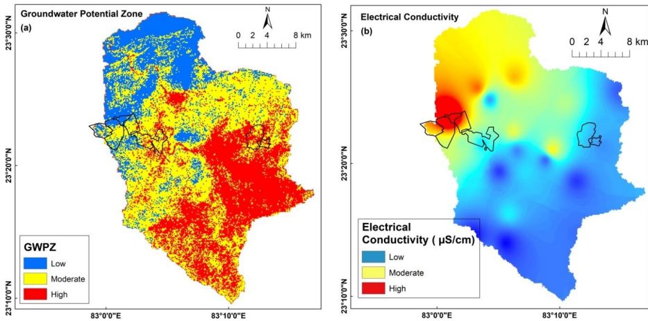
Fig. 3. (a) Groundwater Potential zone map (b) Spatial distribution map of Electrical conductivity
