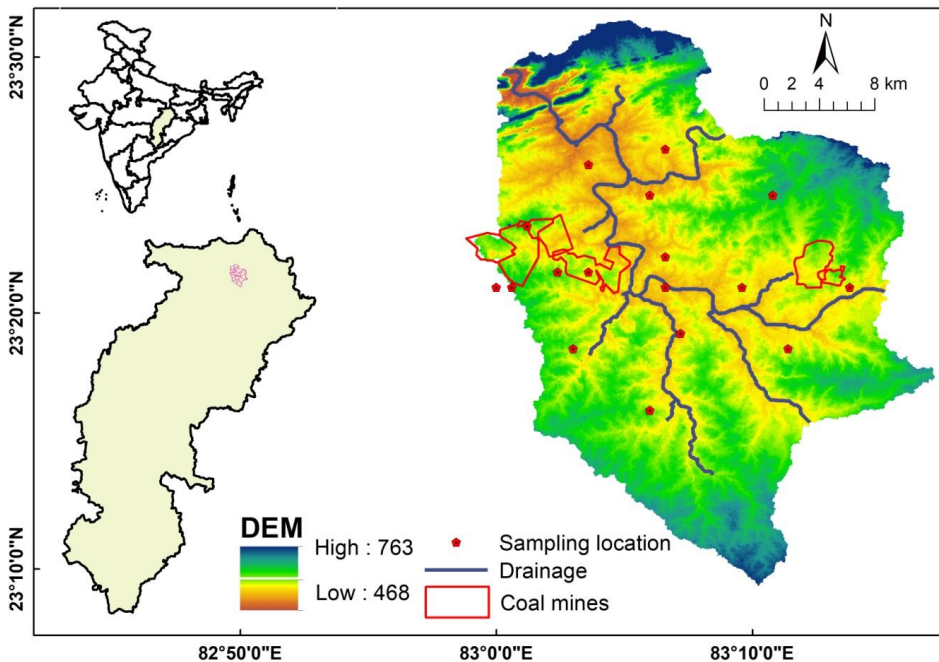
Fig. 1. Study area of Mahan River catchment
