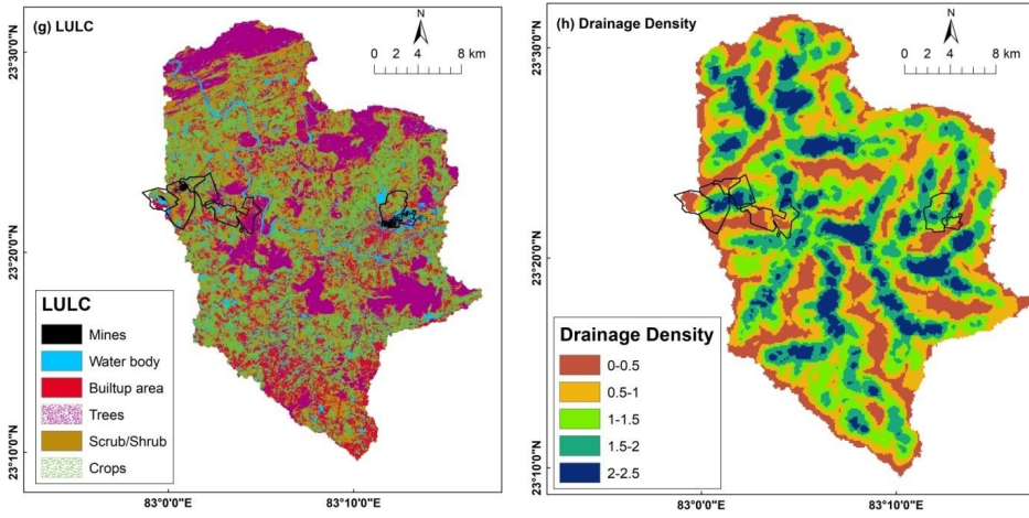
Fig. 2. Thematic maps of the Mahan River catchment area (a) Rainfall (b) Water level (c) Geomorphology (d) Lithology (e) Slope (f) Soil (g) LULC (h) Drainage Density
