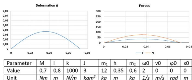
Fig. 15. Simulation results – experiment 6 Own elaboration
