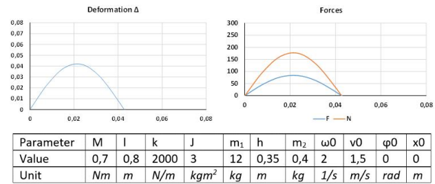
Fig. 10. Simulation results – experiment 1 Own elaboration
