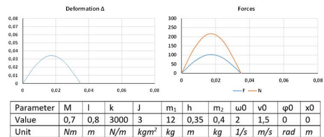
Fig. 11. Simulation results – experiment 2 Own elaboration
