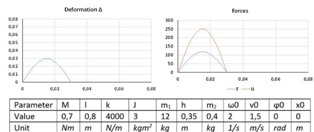
Fig. 12. Simulation results – experiment 3 Own elaboration
