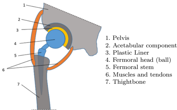
Fig. 4. The model used in the analysis Source: Own elaboration
