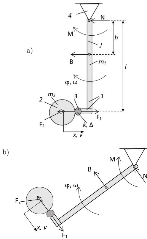
Fig. 8. a, b. Simplifications in model construction Source: Own elaboration
