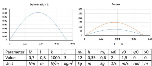
Fig. 14. Simulation results – experiment 5 Own elaboration
