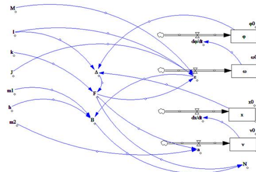
Fig. 9. Structural diagram in Vensim program Source: Own elaboration
