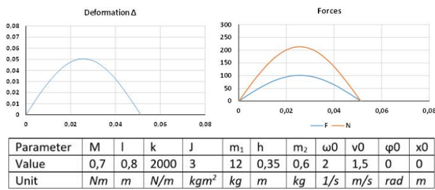
Fig. 13. Simulation results – experiment 4 Own elaboration
