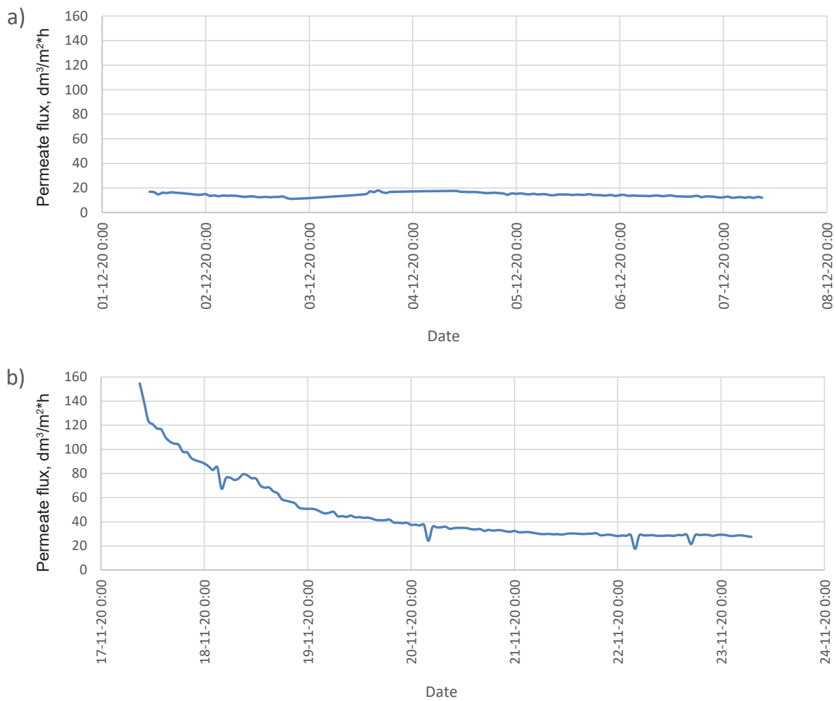
Figure 3. Variability of the permeate flux during the ultrafiltration cycle: a) spiral module (MWCO 200 kDa), and b) capillary module (MWCO 80 kDa).
