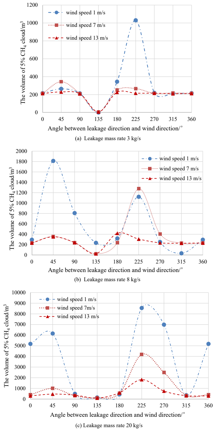
Fig. 11. The variation of stability value of 5% \text{CH}_4 volume at different leakage mass rate and wind speed
