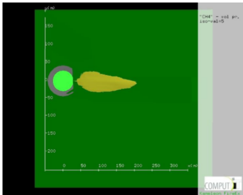
(a) 5%CH 4 volumetric concentration contour line
