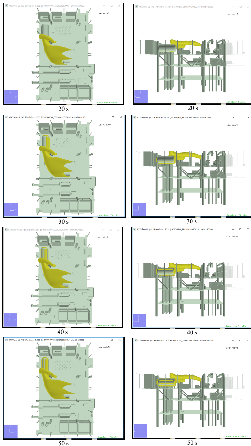
Fig. 6. The spatial and temporal distribution of 5% \text{CH}_4 cloud volume on the platform
