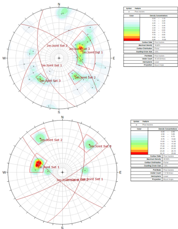
Fig. 17. East and South limb joint sets
