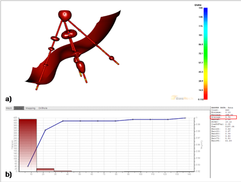
Fig. 13. Q-system for ramp 2_417 mL, a) Borehole analysis, b) Data distribution
