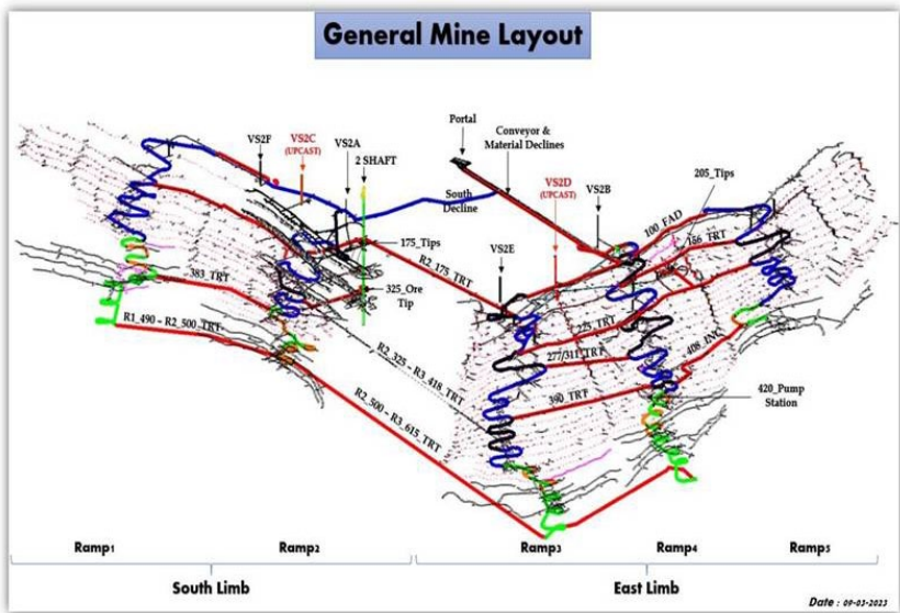
Fig. 4. Ramp 2 general mine lay out
