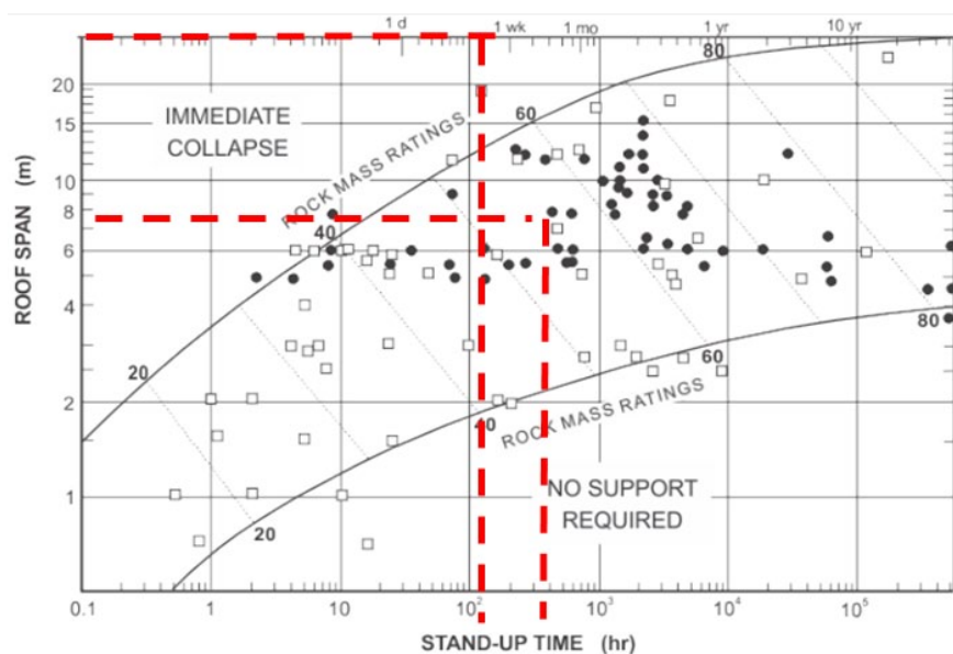
Fig. 15. RMR Stand-up time graph
