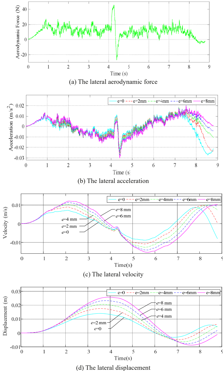
Fig. 9. Simulation results of ascending conveyances in x direction
