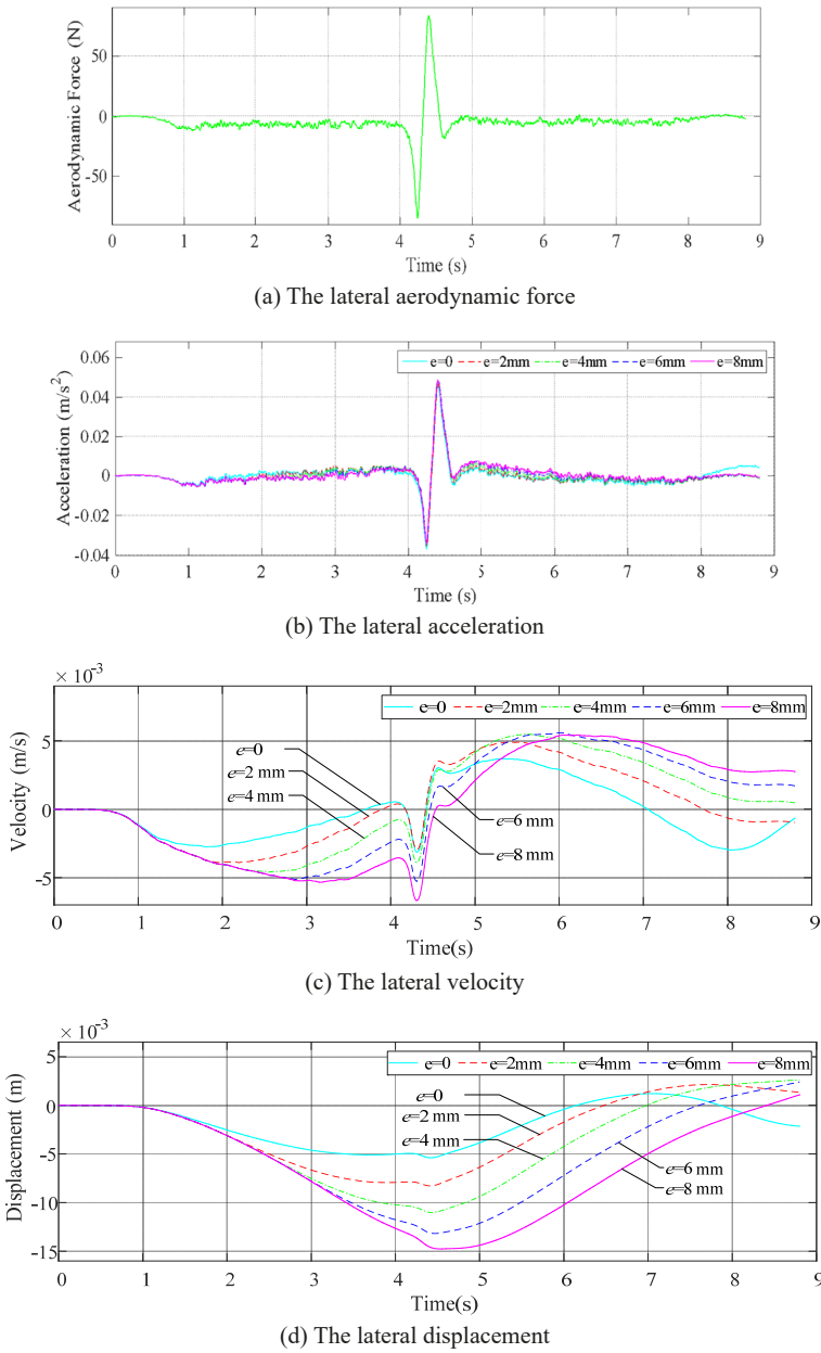
Fig. 10. Simulation results of descending conveyances in x direction
