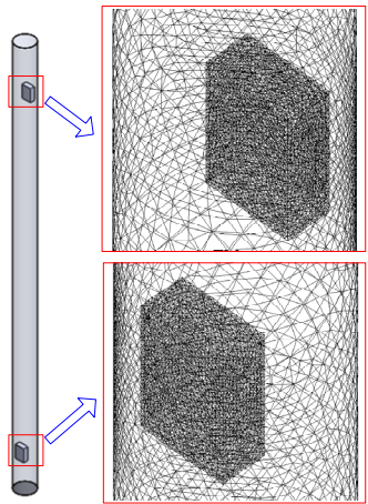
Fig. 6. Meshes used for CFD calculates
