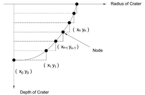
Fig. 4. Estimation modeling of the crater volume
