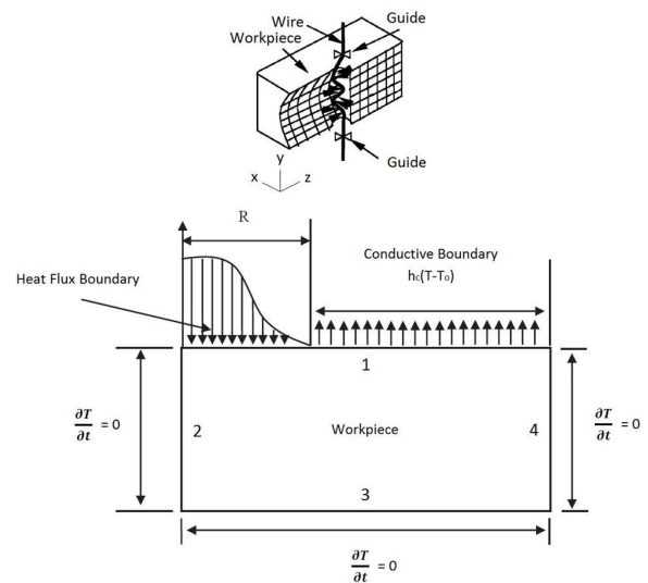
Fig. 3. The WEDM axisymmetric model
