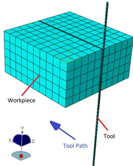
Fig. 2. The workpiece's and tool's undeformed model meshing
