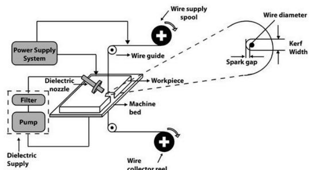
Fig. 1. Schematic diagram of WEDM
