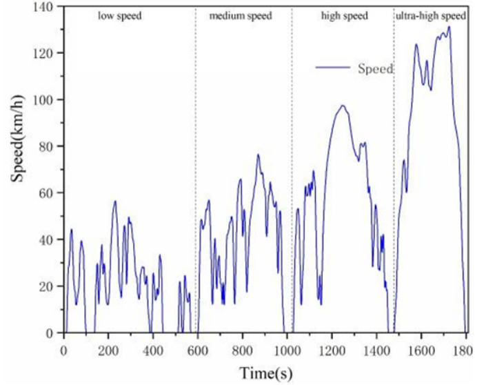
Figure S1. The speed-time relation curve in WLTC
