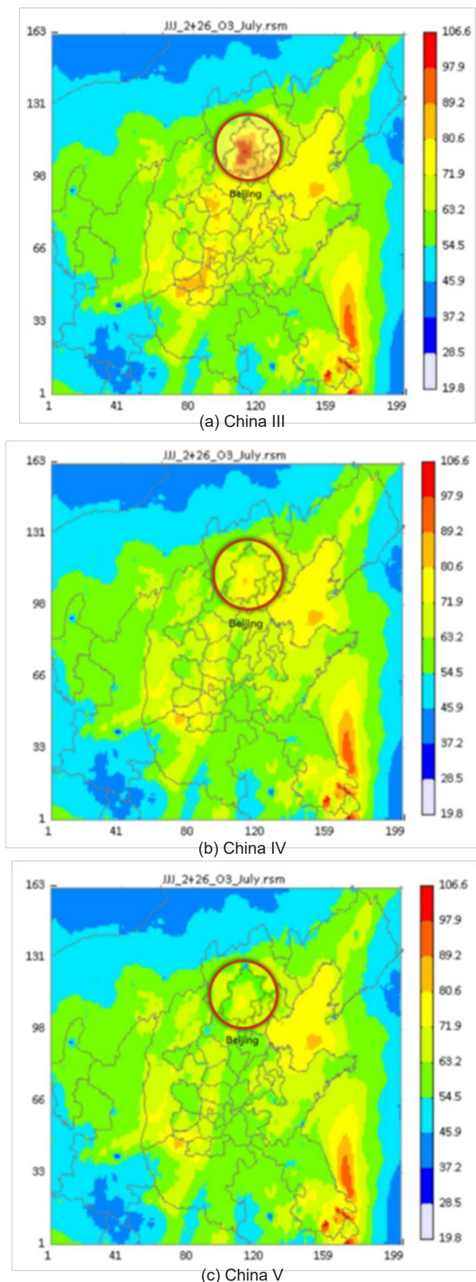
Figure 5. Two-dimensional distribution of O_3 concentration under different emission standard
