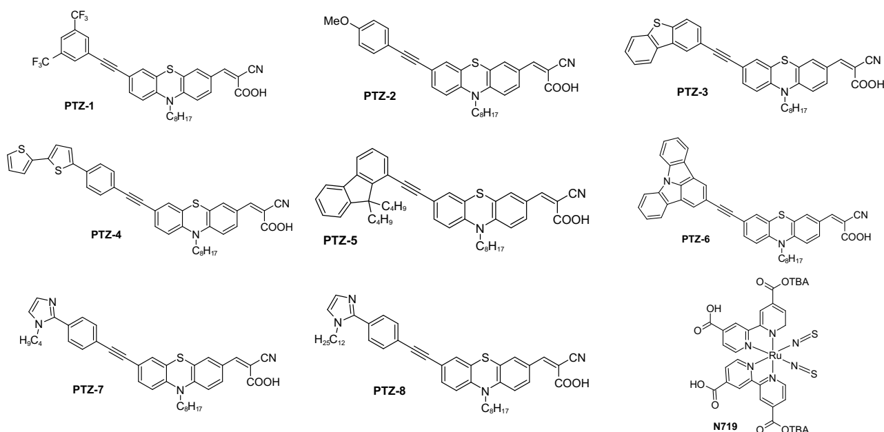
Fig. 1. Chemical structures of phenothiazine derivatives and N719.
