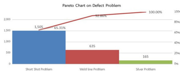
Fig. 4. Pareto chart on defect problem
