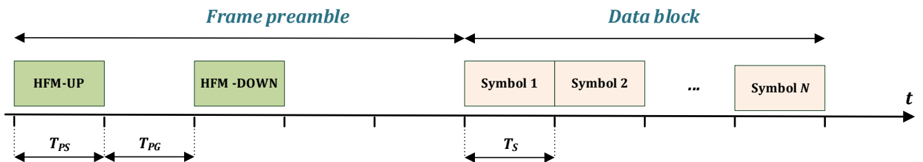
Fig. 2. Frame of transmitted data
