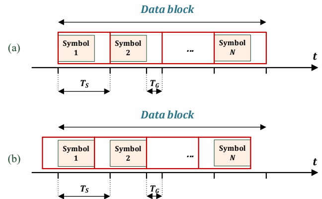
Fig. 6. Analysis window in the frame of transmitted symbols for extreme permissible window shifts \lambda , a) perfectly synchronised analysis window \lambda = 0 , b) analysis window with analysis window shift \lambda = -T_G
