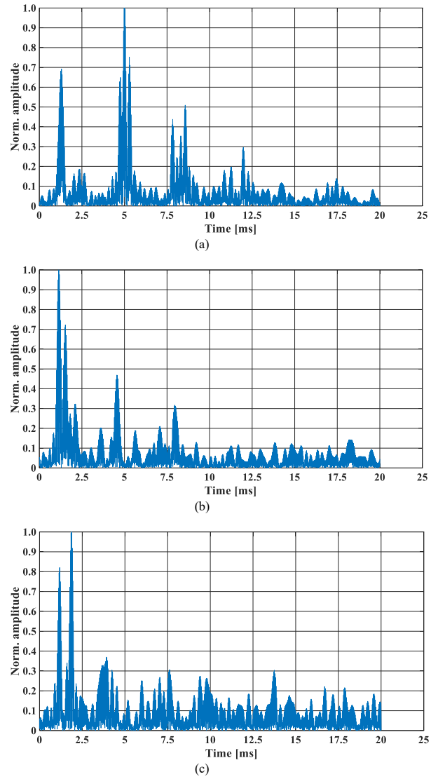
Fig. 10. Impulse response of the shallow-water channel for a transmitter-receiver distance of 250 m (a) hydrophone at the bottom (depth h = 4 ) (b) hydrophone at depth h = 3 (c) hydrophone at depth h = 2
