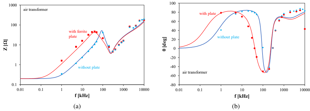
Fig. 6. Measured and computed dependence of the module (a) and phase (b) of the input impedance of the tested air transformers on frequency
