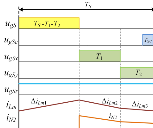
Fig. 3. Switching sequences of ZVS-CSI
