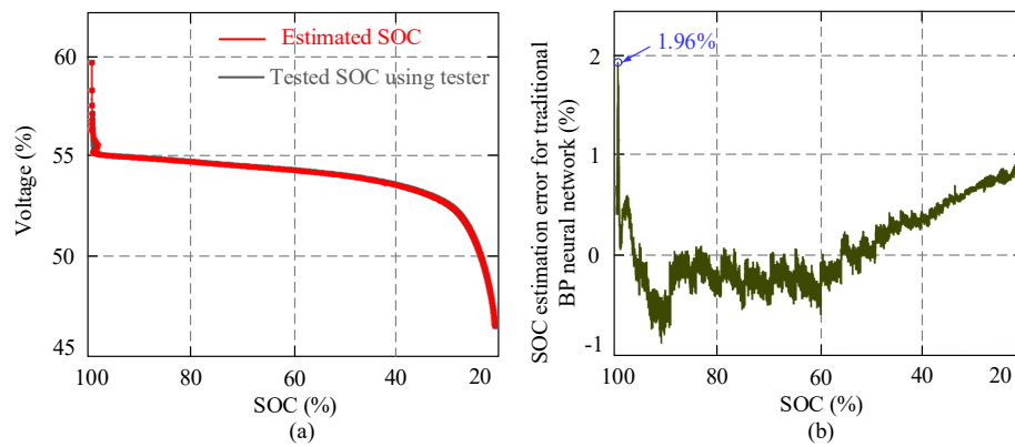
Fig. 12. Estimation results of traditional BP neural network: estimation and tested results (a); SOC estimation error between the estimated and tested results (b)
