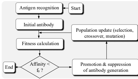
Fig. 5. Implementations of IGA
