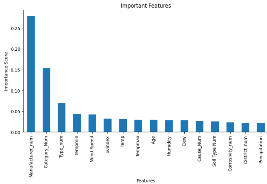
Fig. 6. Feature importance in the equipment failure prediction model
