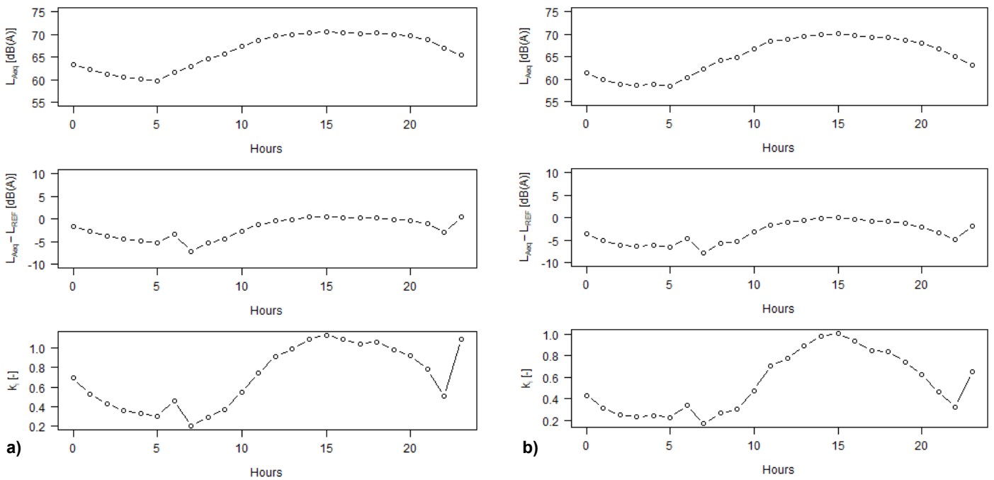
Figure 8. Equivalent sound level L_{Aeq} , exceeding the reference value L_{Aeq} - L_{Aref} and multiplicity factor k_i referenced to 70 dB(A) or 65 dB(A) for Sundays a) in 2016, b) in 2014
