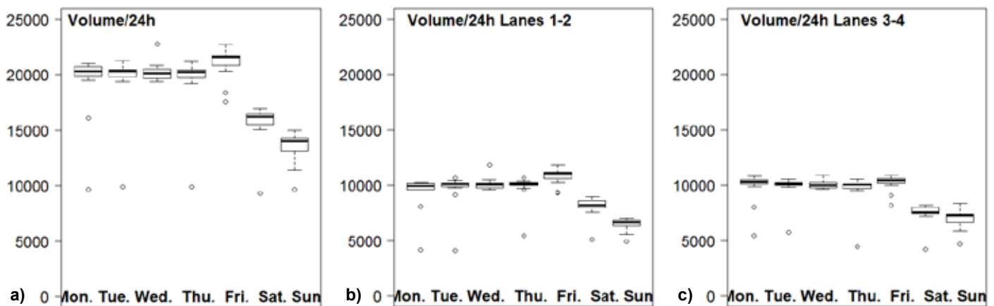
Figure 3. Box plots for annual daily traffic volume determined a) on a section of the road under study, b) on lanes R_{12} , and c) on lanes R_{34} .
