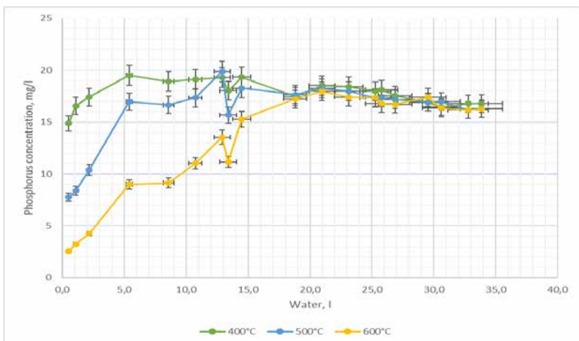
Figure 7. The concentration of phosphate ( \text{PO}_4^{3-}\text{-P} ) during the fixed-bed process using different sewage sludge biochar samples (the lines above each point represent significant differences at p < 0.05 )
