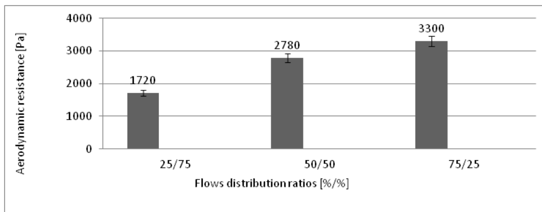
Fig. 7. Six-channel pilot cyclone with a spiral case aerodynamic resistance dependence on the distribution ratio at 12 m/s mean air velocity in the cyclone channels under industrial conditions
