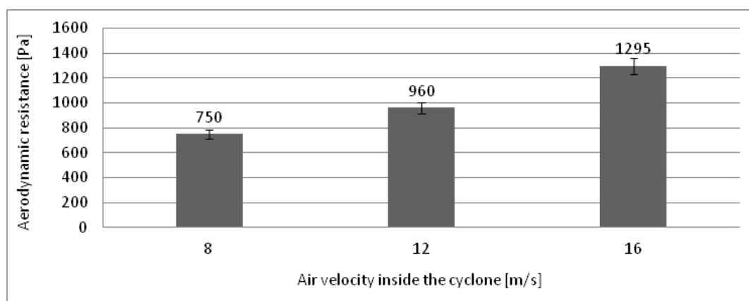
Fig. 5. Dependence of six-channel cyclone aerodynamic resistance on the air flow distribution ratio [50%/50%], under 8 m/s, 12 m/s and 16 m/s mean air flow velocities in the cyclone channels under experimental conditions
