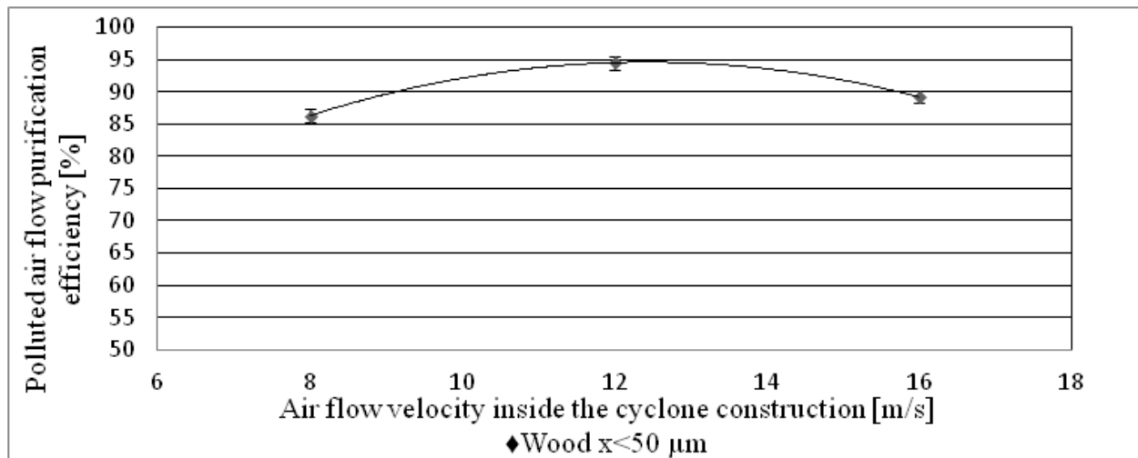
Fig. 6. Air treatment from wood particles, which dispersivity x < 50 \mu\text{m} , efficiency, under the air flow velocity inside the pilot cyclone design, when the air flow distribution ratio is 50%/50% under industrial conditions
