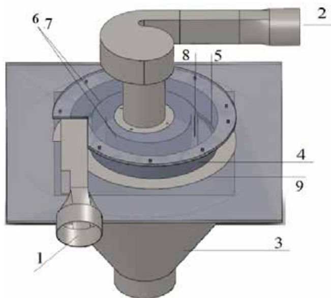
Fig. 1. Spiral multi-channel cyclone with unregulated gaps between the curvilinear semi-rings:
