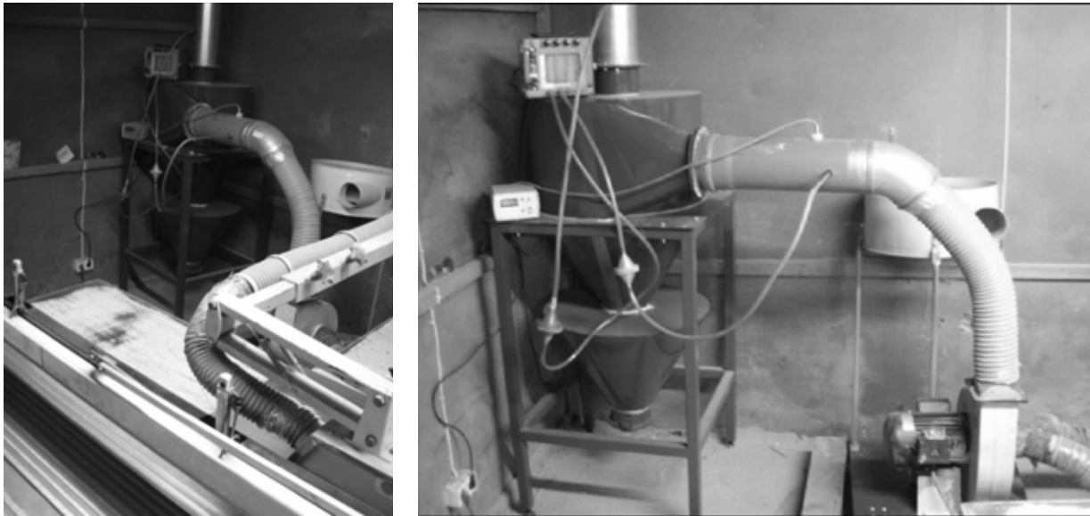
Fig. 3. Studies of the spiral six channel cyclone with adjustable gaps between the curvilinear semi-rings under industrial conditions
