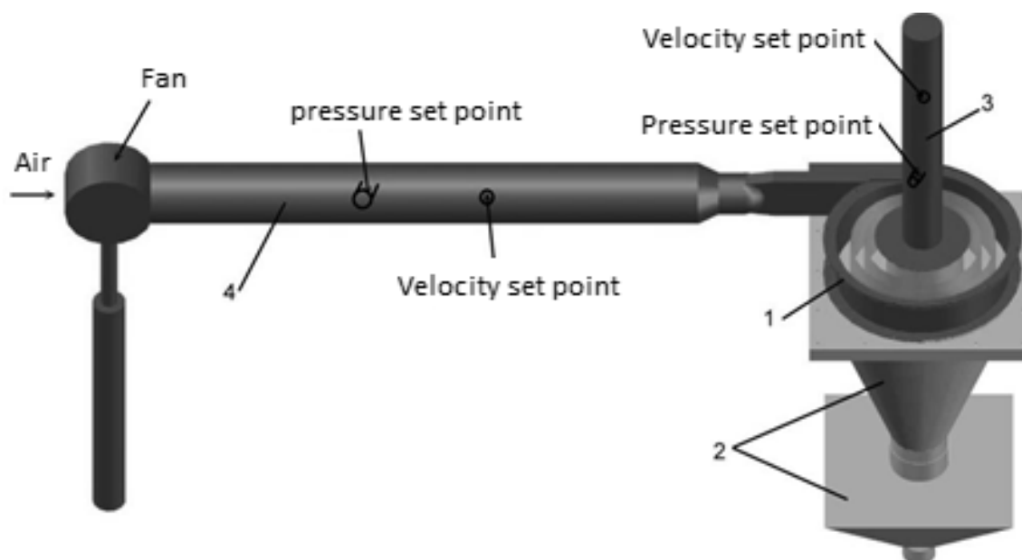
Fig. 2. The six-channel cyclone with adjustable gaps between the curvilinear semi-rings with the spiral case: (1) multi-channel cyclone with a spiral case; (2) double hopper; (3) out air path; (4) duct of polluted air inlet
