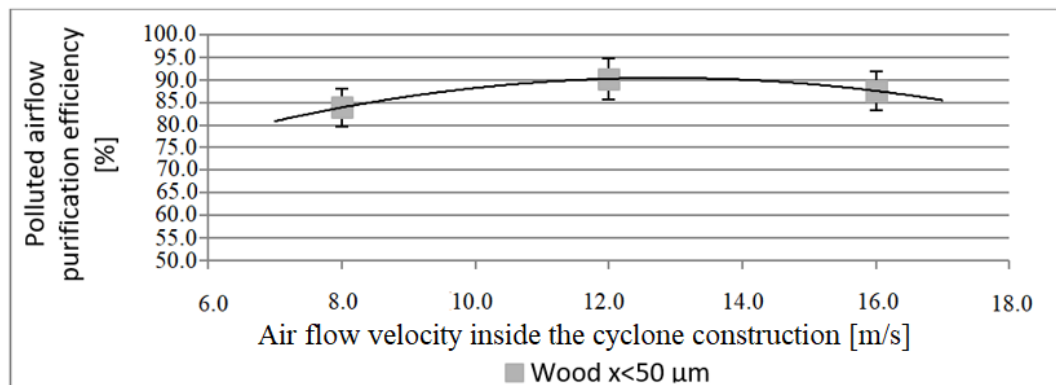
Fig. 4. Air treatment from wood particles, which dispersivity x < 50 \mu\text{m} , efficiency, under the air velocity inside the cyclone design, when the air distribution ratio is 50%/50% under experimental conditions
