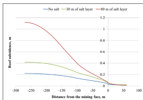
Fig. 9. Roof convergence along the mining direction with different thickness of the salt layer
