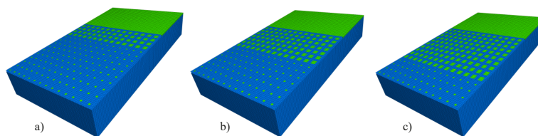
Fig. 8. Numerical model of the rock mass with different widths of the opening front: a) 4 strips, b) 7 strips, c) 10 strips
