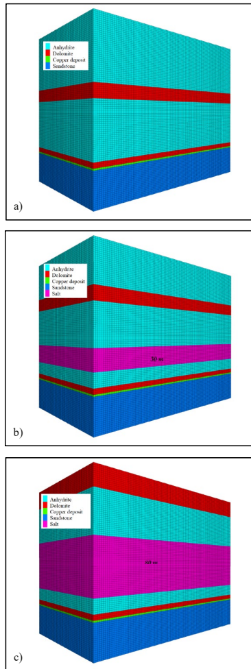
Fig. 7. Numerical model of the rock mass with the assumption related to the presence of salt in the roof: a) no salt, b) 30 m, c) 80 m
