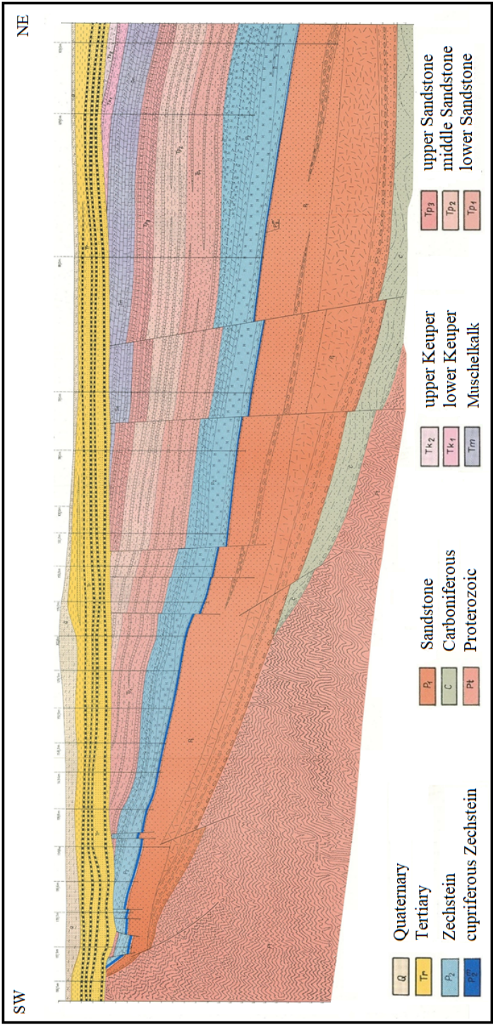
Fig. 4. An example of geological cross-section at the "Polkowice-Sieroszowice" copper ore mine
