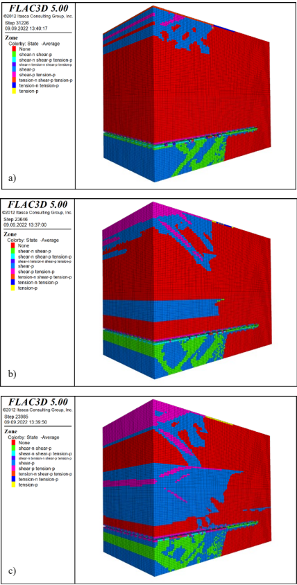
Fig. 10. Plasticity indicators around the mining excavations with different thickness of the salt layer: a) no salt, b) 30 m of salt, c) 80 m
