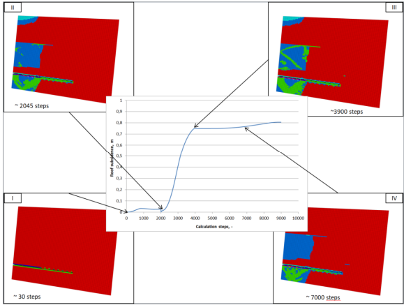
Fig. 11. Convergence and fracture propagation of rock mass in case of 80-m salt layer
