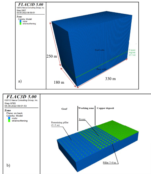
Fig. 5. Numerical model in FLAC3D: a) adopted constitutive models for rock mass, b) actual geometry of the room and pillar system
