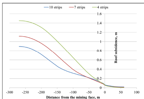
Fig. 12. Roof subsidence along the mining direction with a different width of the opening front (working zone)
