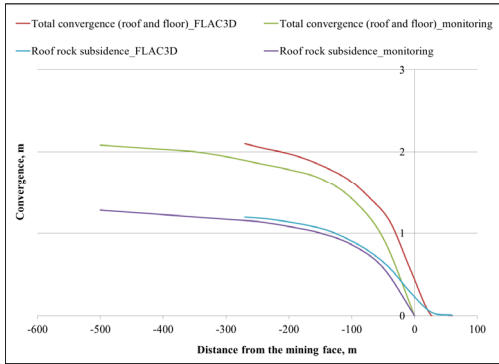
Fig. 6. Comparison of the convergence values along the mining direction with the room and pillar system
