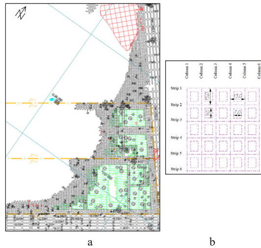
Fig. 2. The room and pillar system at the SI-XII mining field: a) Outline of the room and pillar system with the roof layers deflection; b) Dimension of rooms and pillars
