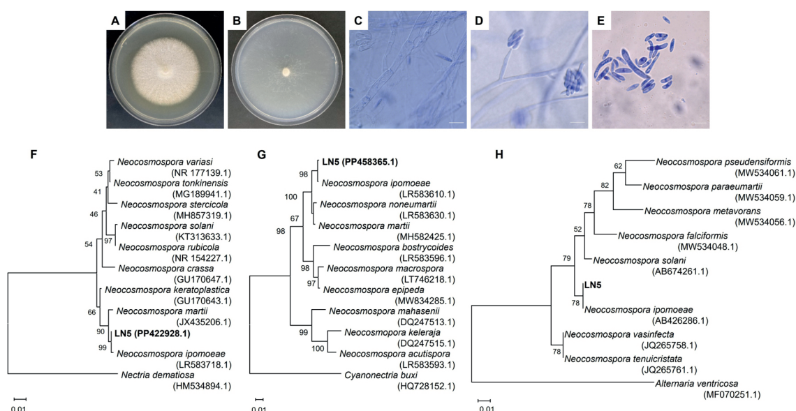
Fig. 4. Morphology and taxonomic position of strain LN5. A – colony on PDA; B – colony on LCA; C – septate mycelia; D – unbranched conidiophore; E – macro- and microconidia. Scale bars 10 µm. F, G, H – phylogenetic trees based on comparative analyses of the ITS, TEF1, and BT2 sequences, respectively (accession numbers of these sequences are indicated in parentheses next to the strain name)
