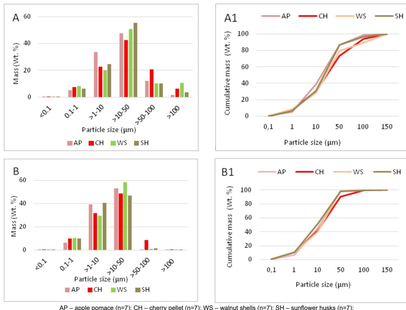
Figure 1 Granulometric composition of the produced ashes: A - particle size distribution and A1 - cumulative curve of the percentage of grain size (400±15°C); B - particle size distribution, B1 - cumulative curve of the percentage of grain size (850±15°C)
