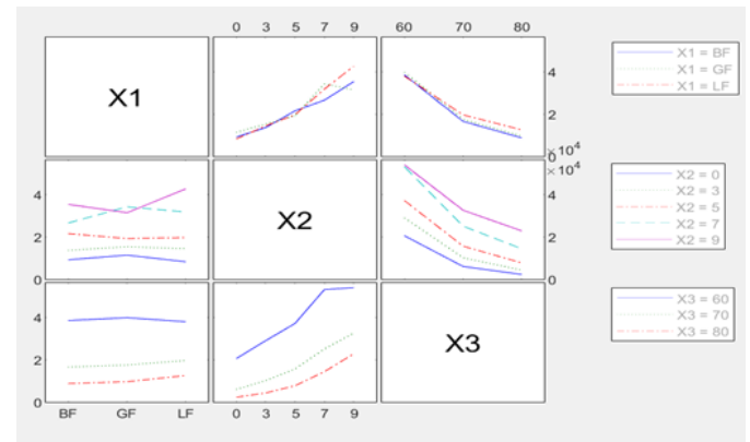
Fig. 7. Correlation of rutting factor RF with applied filler X1, SBS copolymer content X2, and measurement temperature X3 for RTFOT-aged mastics
