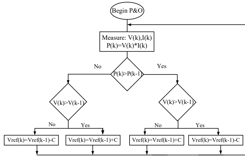
Fig. 1. Flow chart of the P&amp;O algorithm
