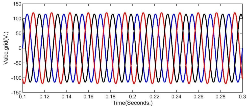
Fig. 16. Voltage of the three-phase grid under unbalanced grid voltage
